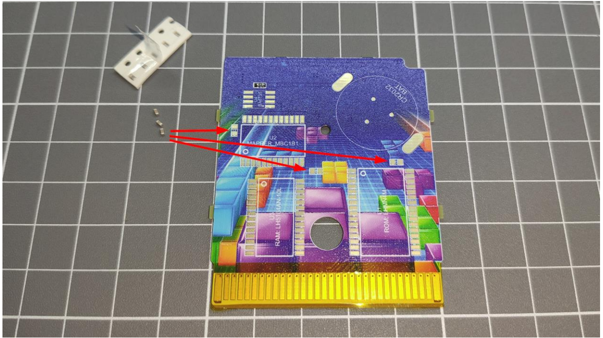
Capacitors installation (Board version 1.1)
